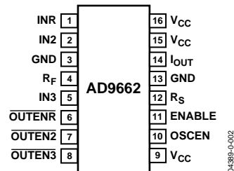
Figure 2. QSO-P-16 Pinout
